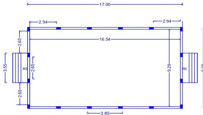
PLAN SCALE 1:100
