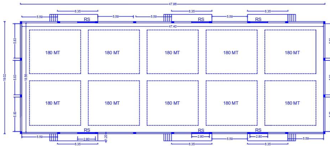
PLAN FOR 1800 MT WAREHOUSE SCALE 1:100
